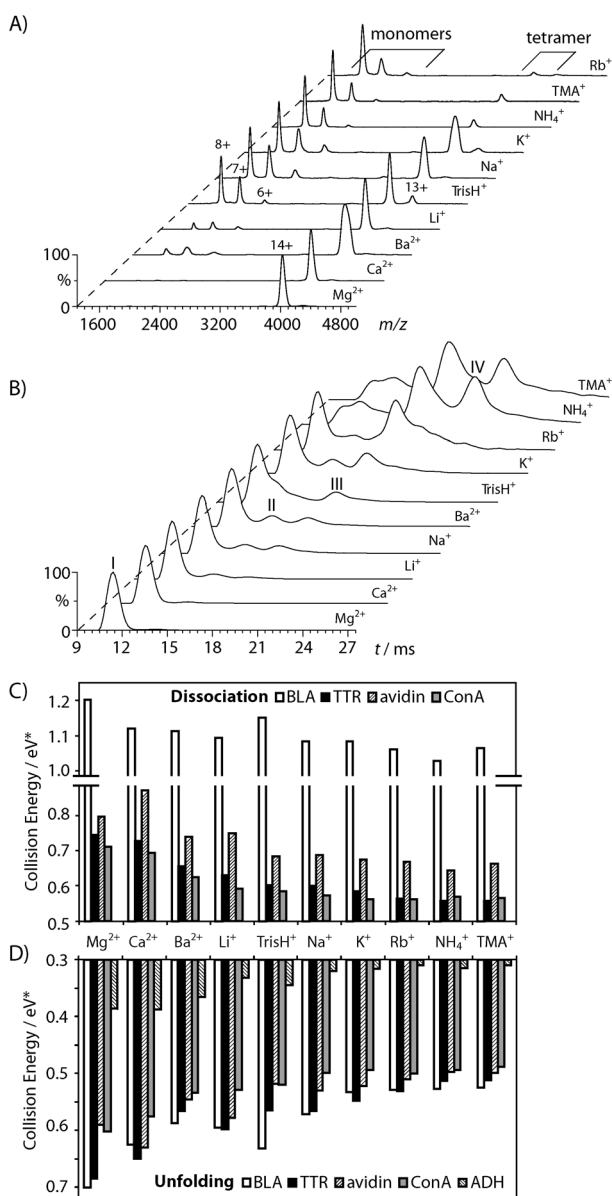
Figure 1. A) MS data for 14^+ TTR incubated with ten cations of acetate salts at 60 V trap collision voltage. The data also contain signals corresponding to 6 – 8^+ charge state monomers, resulting from CID of the complex. B) IM data for the same cations shown in (A), at 55 V trap collision voltage. Four distinct drift time features are labeled I–IV. Histogram plots of collision energy ( \text{eV}^* ) required to dissociate (C) and unfold (D) 50% of the population of dimeric BLA and tetrameric TTR, avidin, ConA, and ADH are shown for a range of cation additives. Control data sets are also marked on the plot ( \text{NH}_4^+ ).
